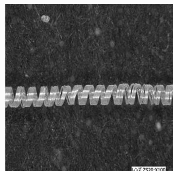
Crimp structure
